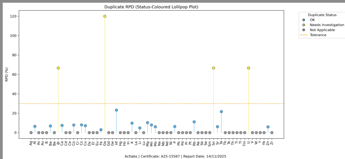
Automated Lab Internal QC Evaluation Report from GitHub
